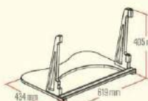
Floor Stand (Tilt) •Weight : 21.28 kg • Fixed 5° tilt angle
